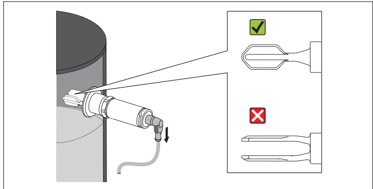
Figure 5.9 Position of the fork in the case of horizontal installation in a vessel
