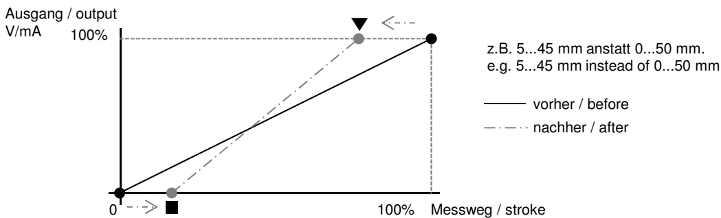
Kennlinie / characteristic 1: Null- und/oder Endpunkt einstellen / Setting up zero- and/or limit point .
