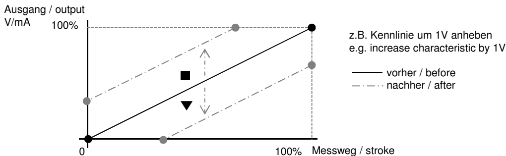
Kennlinie / characteristic 3: Offset einstellen / setting up offset
