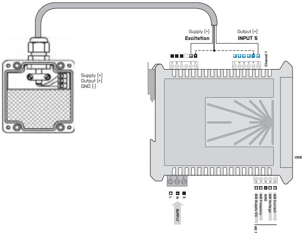
Example connection of a 3-wire sensor with current signal output powered by instrument's excitation
