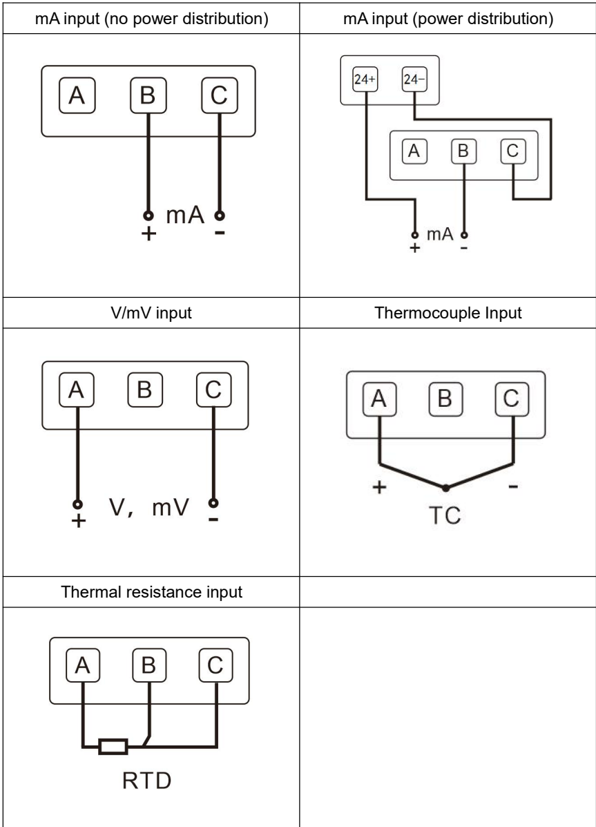
Fig. 2-4 Schematic diagram of signal line connection
