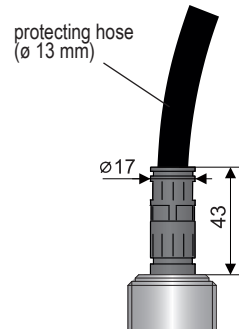
Variant "H" with cable gland for protecting hoses - for use in an outdoor area or in area with high humidity.
