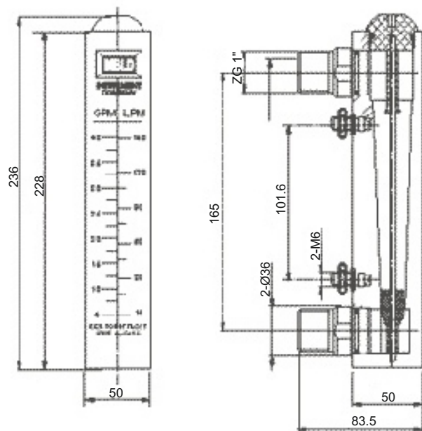
LZT-40__M (4035M, 4040M)
