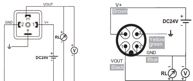
3-wire voltage output
