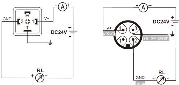
2-wire 4mA - 20mA output
