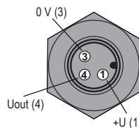
Top view of the connector
