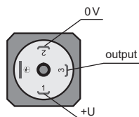
Top view of the connector
