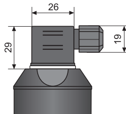
Performance „G” with valve connector
