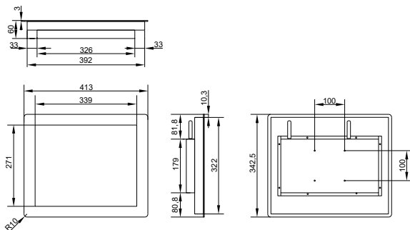
Рисунок 3 – Габаритные размеры / Figure 3 – Overall dimensions / Сурет 3 – Габариттік өлшемдері ICW-F-19-1-1S-170CS-00001, ICW-F-19-1-2S-170CS-00001, ICW-F-I3-1-1S-170CS-00001, ICW-F-I3-1-2S-170CS-00001, ICW-F-I5-2-3S-170CS-00001, ICW-F-I5-3-3S-170CS-00001, ICW-F-I7-3-4S-170CS-00001, ICW-F-19-1-1S-170CS-00002, ICW-F-19-1-2S-170CS-00002, ICW-F-I3-1-1S-170CS-00002, ICW-F-I3-1-2S-170CS-00002, ICW-F-I5-2-3S-170CS-00002, ICW-F-I5-3-3S-170CS-00002, ICW-F-I7-3-4S-170CS-00002
