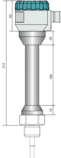
High temperature performance CLM-70_T**
