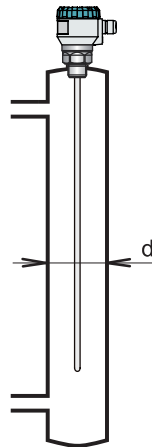
Fig. 1: Installation of level meters with rod electrodes
