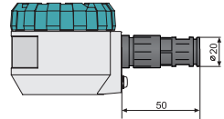
Variant CLM-70 with a cable gland for protective hose
