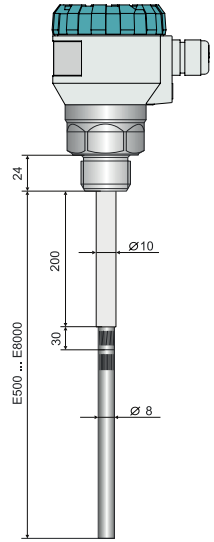
Variant CLM-70 with a cable gland for protective hose
