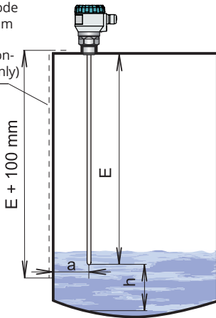
Fig. 1: Installation of level meters with rod electrodes
