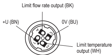
Inside view of the connector socket (variant "C-PFPT")
