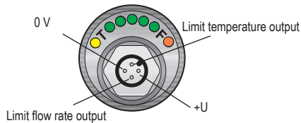
Connector of flow sensor TFS-35_--_--PFPT
