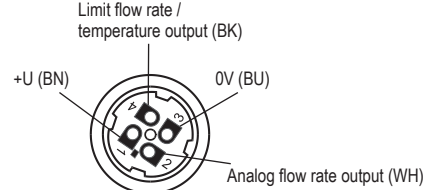
Inside view of the connector socket (variant "C-IFPP(P)")
