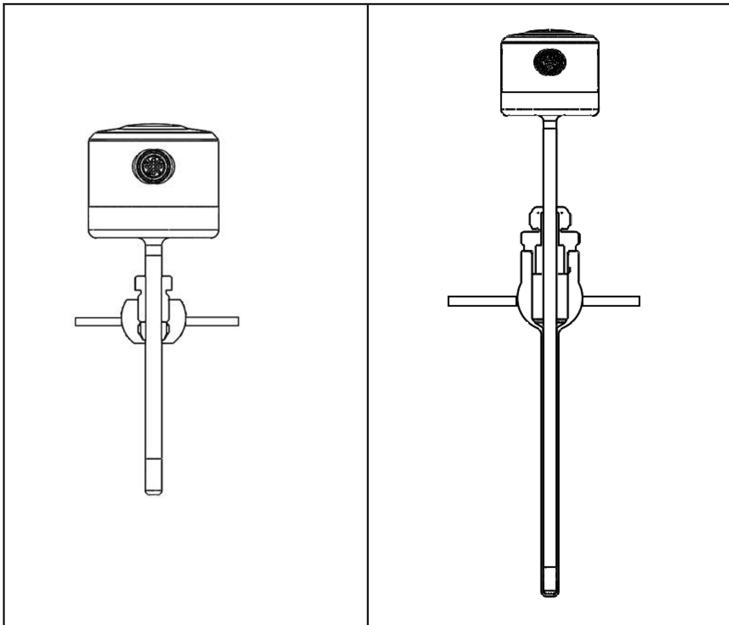
Fig. 2: direct installation (e.g. with adapter E30407)
