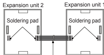
Cable length: max. 1m
