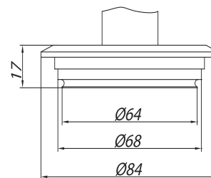
Varivent
